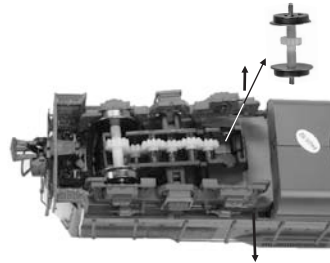
Separate the truck sides in order to free the drive wheel
