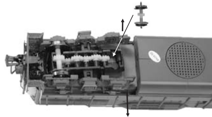
Separate the truck sides in order to free the drive wheel
