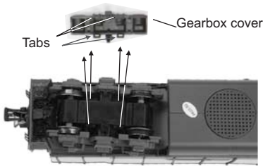
Pry the tabs inward to detach gearbox
