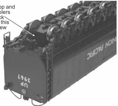
Figure: Installing the Hook and Loop type coupler.
