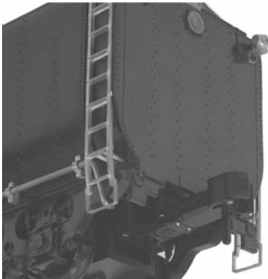
Figure: MTH ProtoCoupler in higher position.
