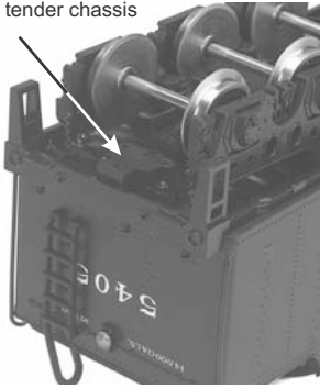
Install Kadee Coupler Mount into mounting holes on tender chassis
