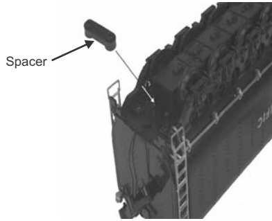
Figure: Add Spacer and reattach ProtoCoupler
