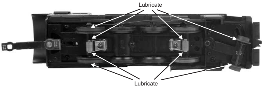
Figure 8: Lubrication Points
