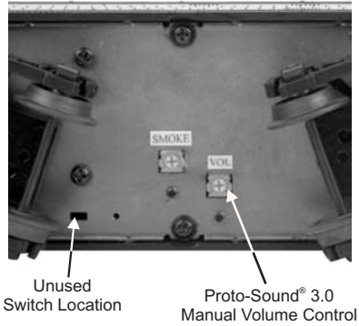
Figure 7: Manual Volume Control
