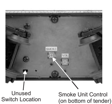
Figure 9: Smoke Unit Control
