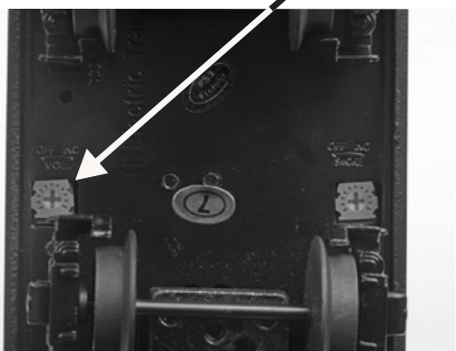
Figure 7: Manual Volume Control
