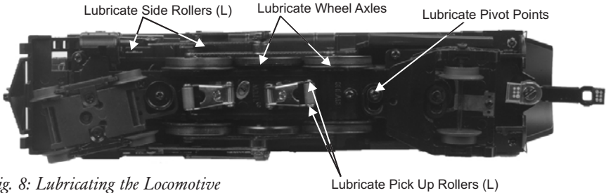
Fig. 8: Lubricating the Locomotive
