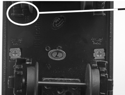
Figure 6: Changing from DCS to DCC Mode
