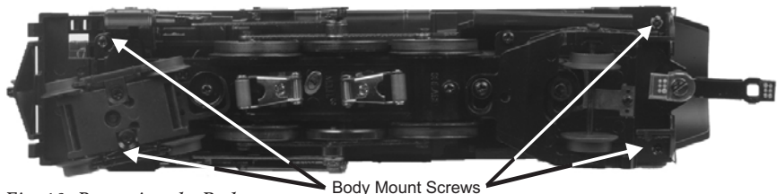
Fig. 10: Removing the Body
