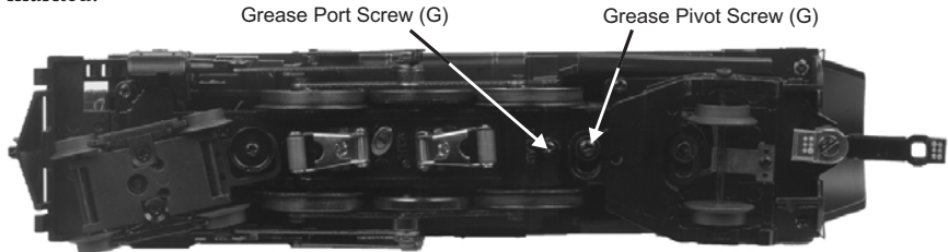
Fig. 9: Grease Points
