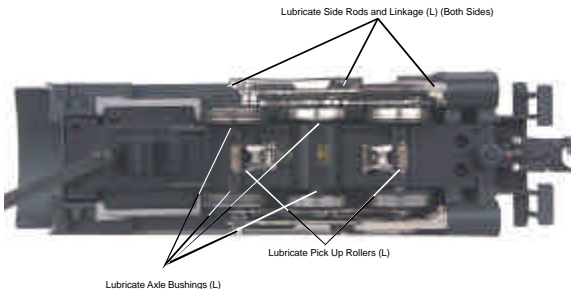
Figure 1. Lubrication Points on the Locomotive
