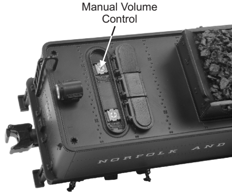
Figure 7: Manual Volume Control
