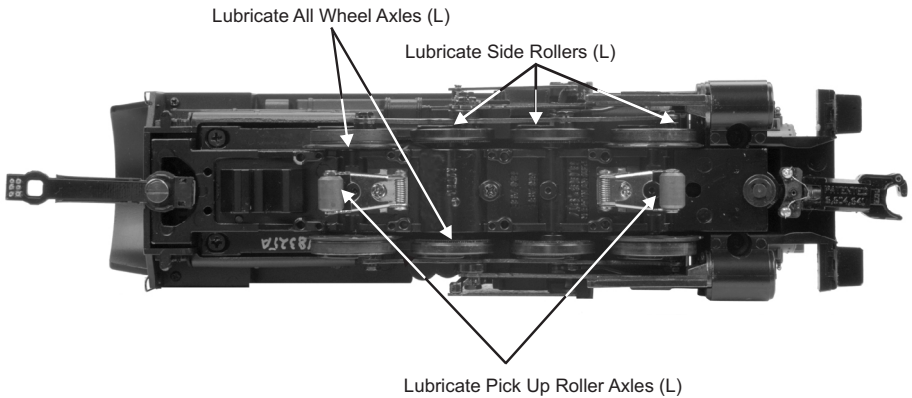
Figure 8: Lubricating the Locomotive
