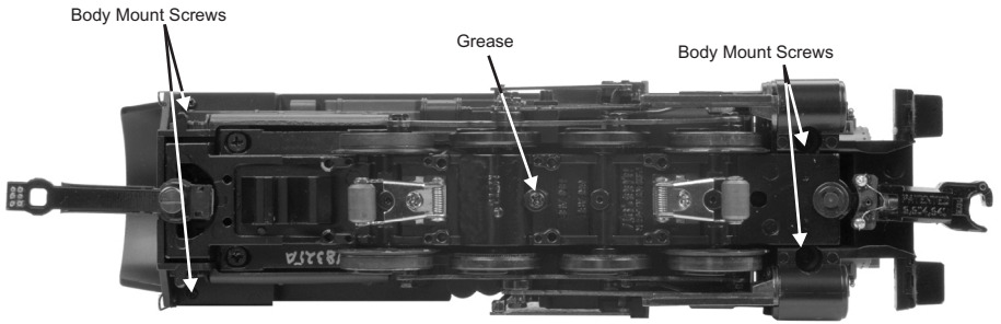
Figure 9: Body Mount Screws and Grease Points
