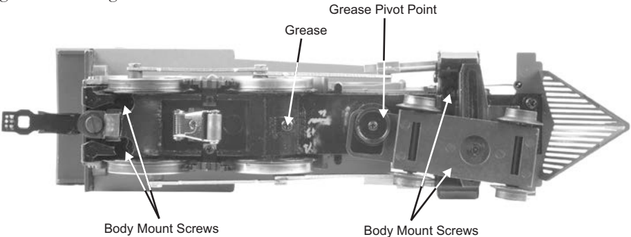
Figure: Body Mount Screws and Grease Points
