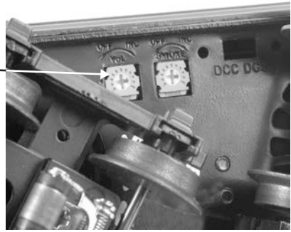
Figure: Manual Volume Control
