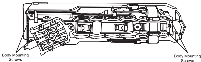
Figure 10: Removing The Boiler From The Chassis
