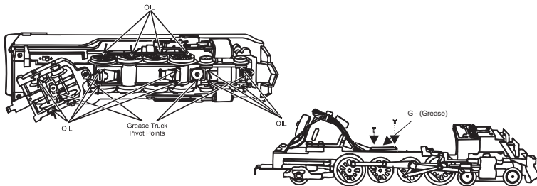
Figure 8: Lubricating The Locomotive Chassis
