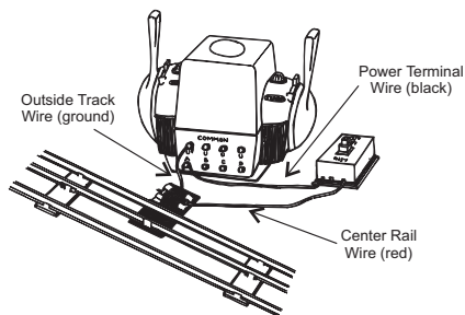
Figure 7: Wiring Up A Bell Button
