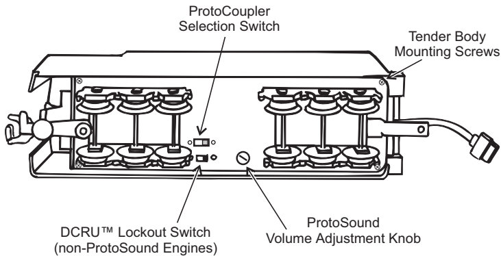
Figure 6: Adjusting The ProtoSound® Volume
