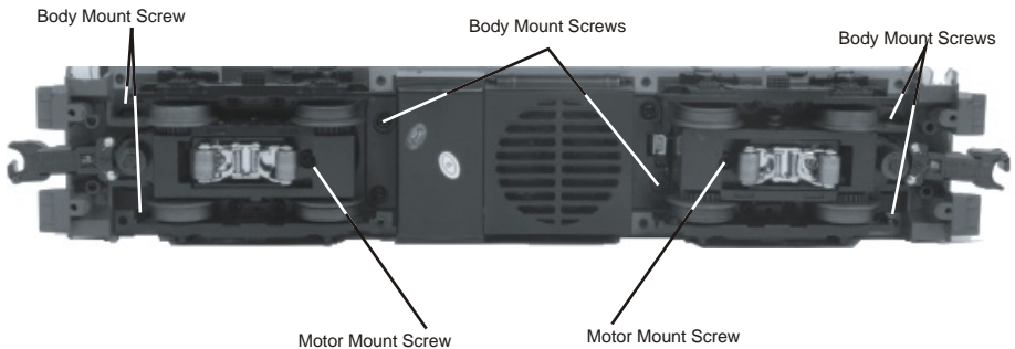
Figure 4: Mounting Screws
