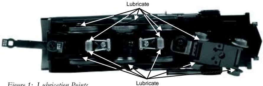
Figure 1: Lubrication Points
