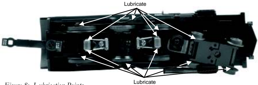
Figure 8: Lubrication Points
