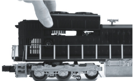
Figure 2a. Remove Fan Cover to Access Smoke Unit and Volume Controls
