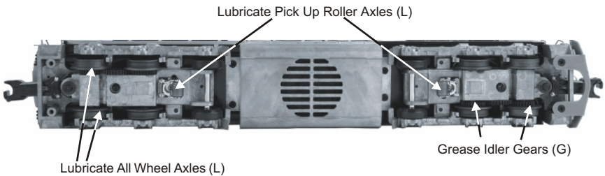
Figure 5: Lubrication Points
