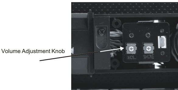
Figure 4: Volume Adjustment
