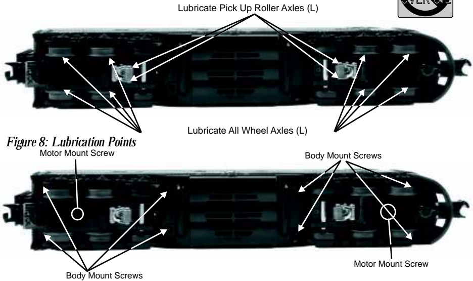
Figure 9: Body Removal Screw Locations and Motor Mounting Screws
