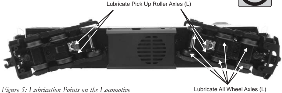
Figure 5: Lubrication Points on the Locomotive
