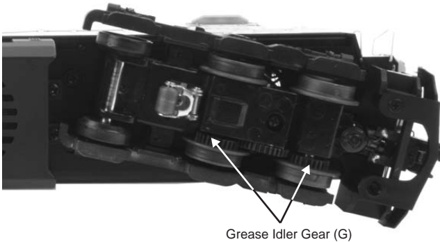
Figure 7: Greasing the Idler Gears
