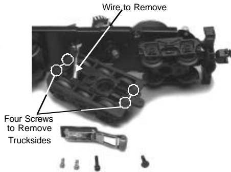
Figure 4b. Locating the wire to remove and the four truck mounting screws
