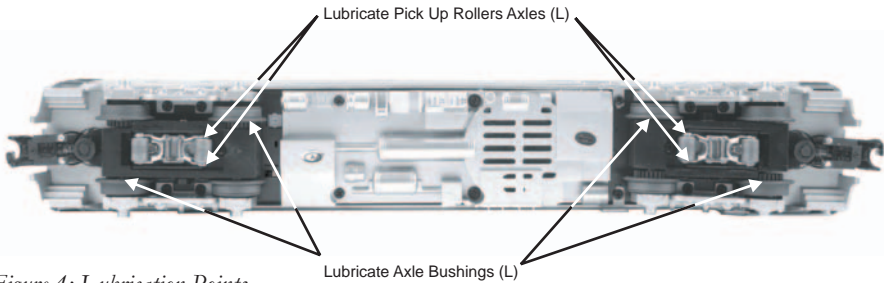
Figure 4: Lubrication Points
