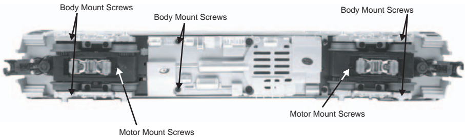
Figure 5: Body Removal Screw Locations and Motor Mounting Screws
