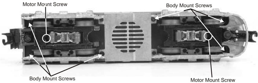
Figure 4. Body Removal Screw Locations
