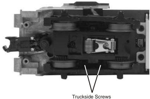
Figure 6. Truckside Screws (Reference Picture Only- Actual Model May Look Different)
