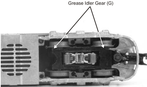
Figure 5. Greasing The Idler Gears
