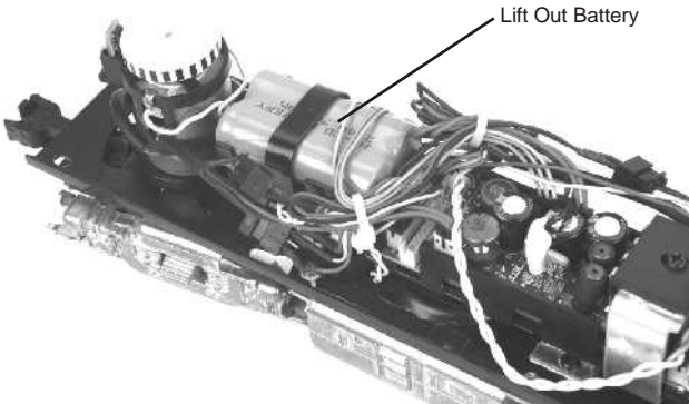
Figure 8. Battery Location.
