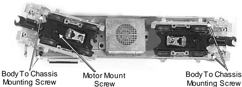
Figure 7: Lubricate The Tender Chassis Trucks
