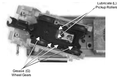
Figure 6: Lubricating The Locomotive Chassis
