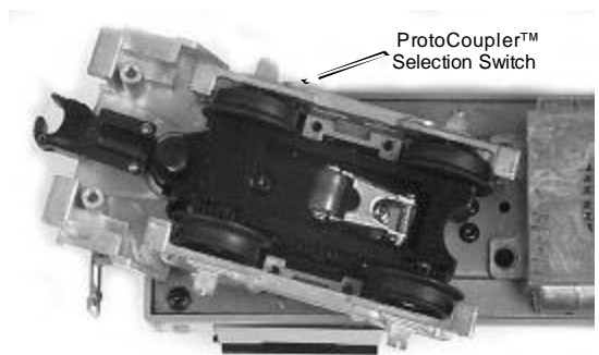
Figure 5: Proto-Coupler Selection Switch
