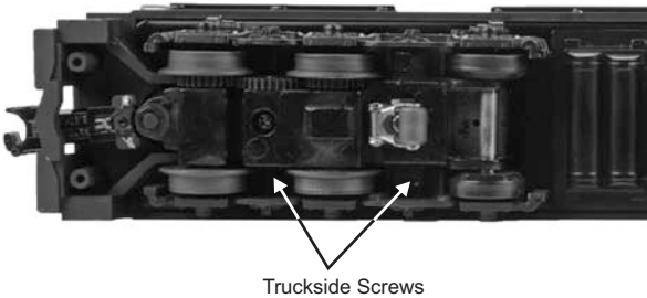
Figure 9: Truckside Screws
