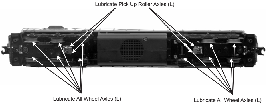
Figure 6: Lubrication Points on the Locomotive
