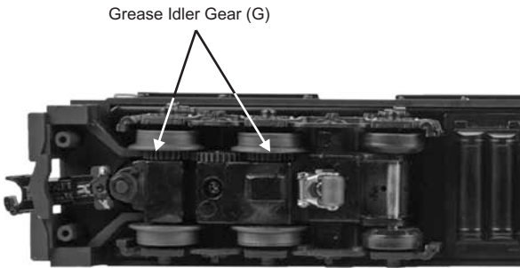
Figure 8: Greasing the Idler Gears
