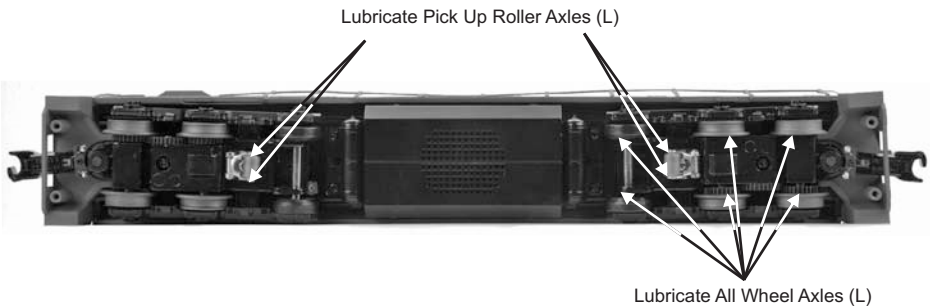
Figure: Lubrication Points on the Locomotive
