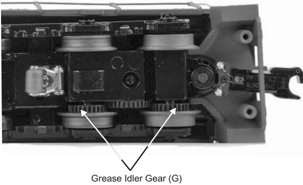
Figure: Greasing the Idler Gears
