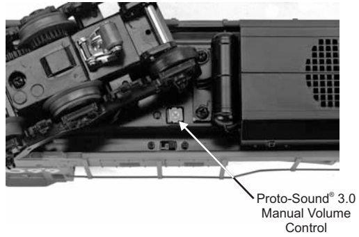
Figure: Manual Volume Control
