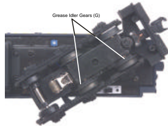
Figure 6: Greasing The Idler Gears
