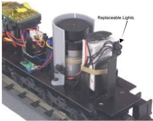
Figure 7: Removing The Replaceable Lights
