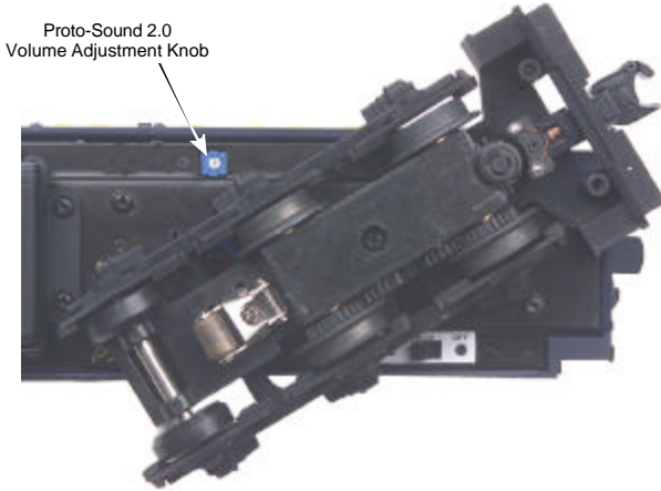
Figure 4: Manual Volume Adjustment Knob
