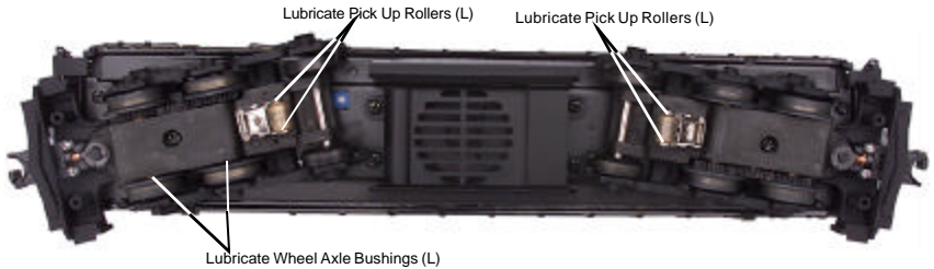
Figure 2. Lubrication Points on the Engine
