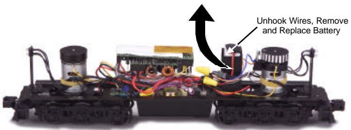
Figure 6. Removing and Replacing the Battery
