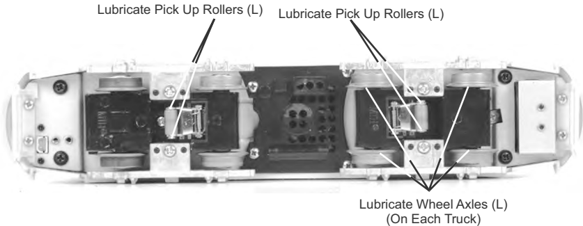
Figure: Lubrication Points on the Locomotive
