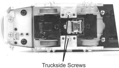
Figure: Truckside Screws
