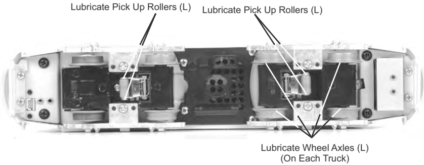
Figure: Lubrication Points on the Locomotive
