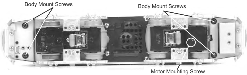
Figure: Body Mount and Motor Mount Screws
