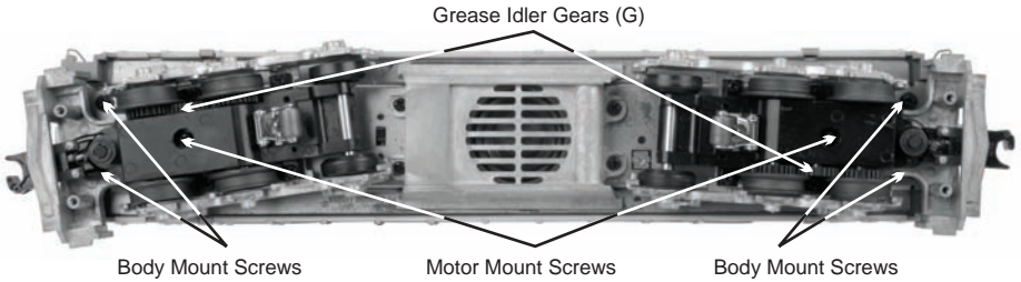
Figure 6: Body Mount Screws and Grease Points
