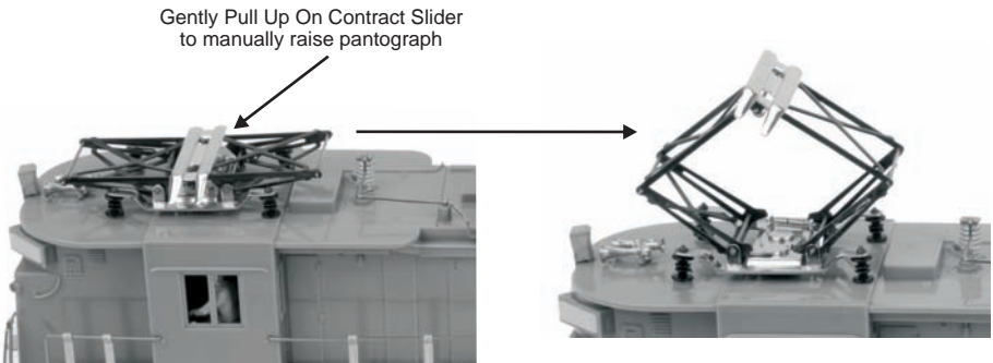
Figure 2: Unlatching Pantographs
