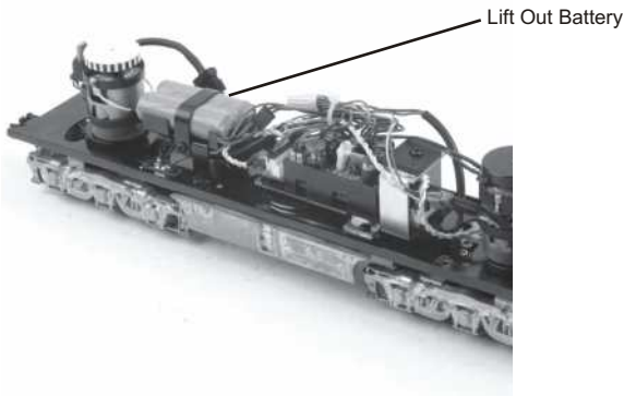
Figure 8. Battery Location.
