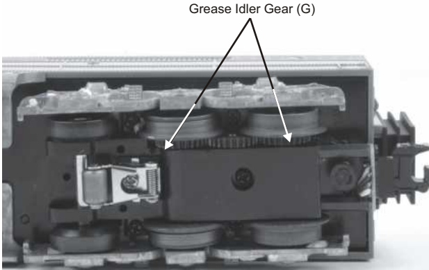
Figure 5. Greasing The Idler Gears
