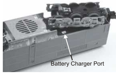
Figure 7. Battery Charger Port Location.
