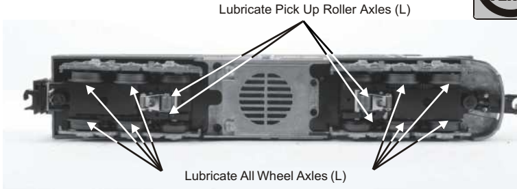
Figure 3. Lubrication Points on the Locomotive
