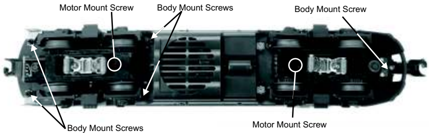
Figure 10: Motor Mount and Body Mount Screws
