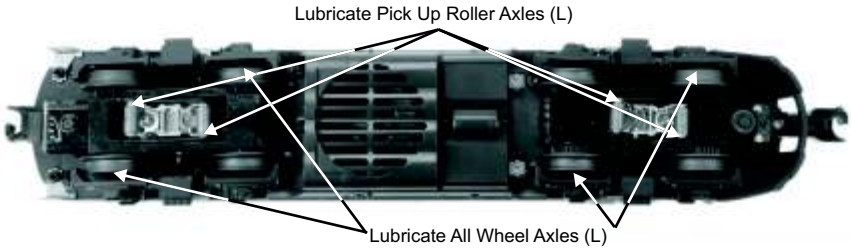
Figure 9. Lubrication Points on the Locomotive
