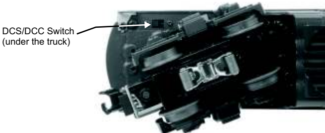
Figure 7: Changing from DCS to DCC Mode
