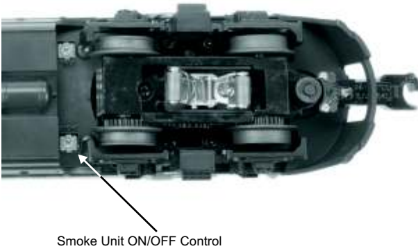
Figure 3. Smoke Unit Control
