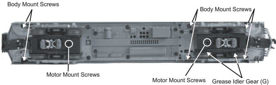
Figure 5. Body Removal Screw Locations
