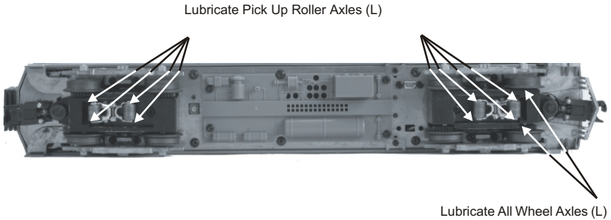
Figure 1. Lubrication Points on the Locomotive
