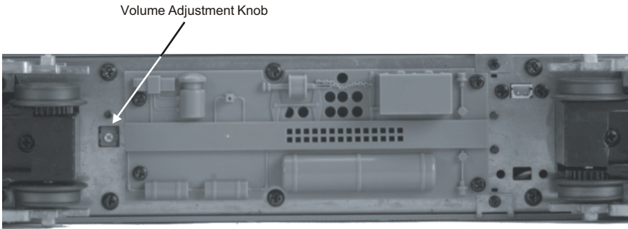
Figure 4. Manual Volume Adjustment Knob
