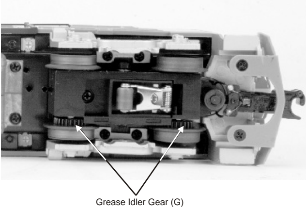
Figure 6. Greasing The Idler Gears
