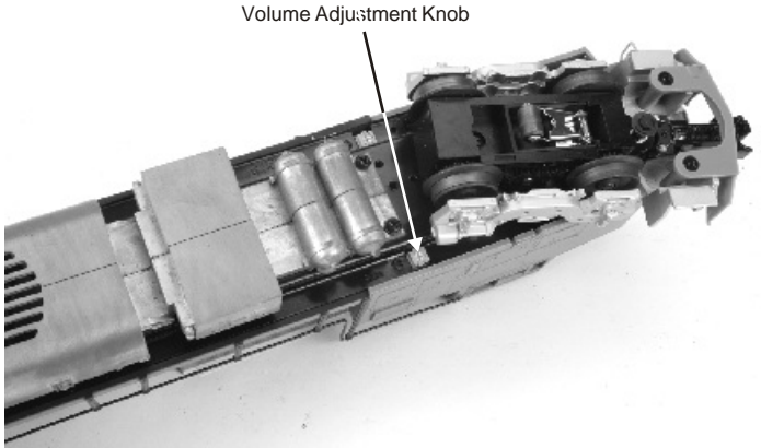
Figure 4. Manual Volume Adjustment Knob
