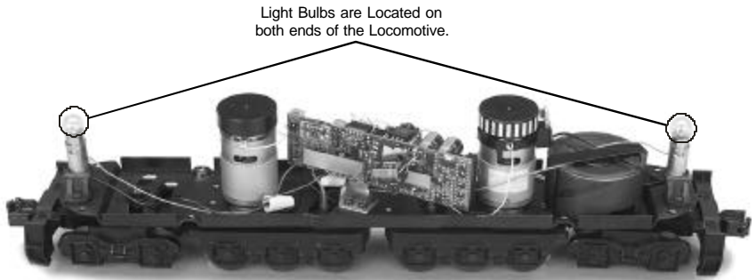
Figure 5. Locate the Burned-Out Lightbulbs in the Locomotive. To Replace the Bulb, turn the Bulb Counter-Clockwise to remove and Install a New One.
