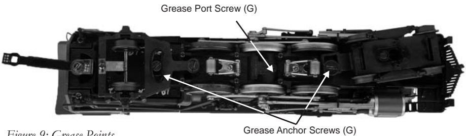
Figure 9: Grease Points
