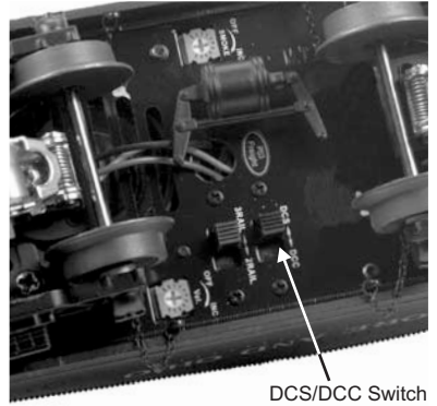
DCS/DCC Switch
