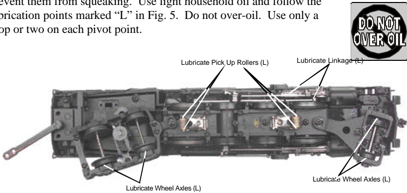
Figure 5: Lubricating The Chassis
