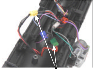
Wires for headlight & marker lights
