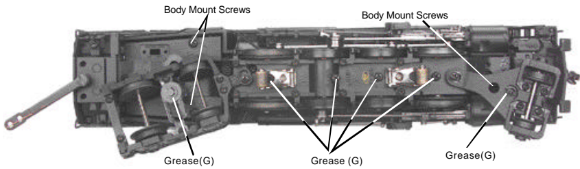
Figure 6: Removing The Body
