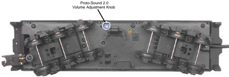
Figure 4: Manual Volume Adjustment
