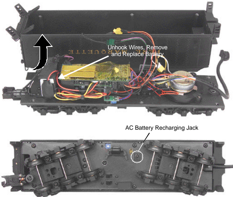
Figure 11: Replacing The Battery And Locating The Battery Recharging Jack
