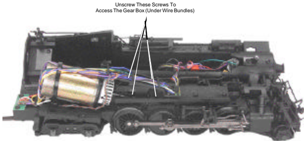
Figure 7: Opening The Gearbox
