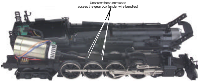
Figure 7: Opening The Gearbox
