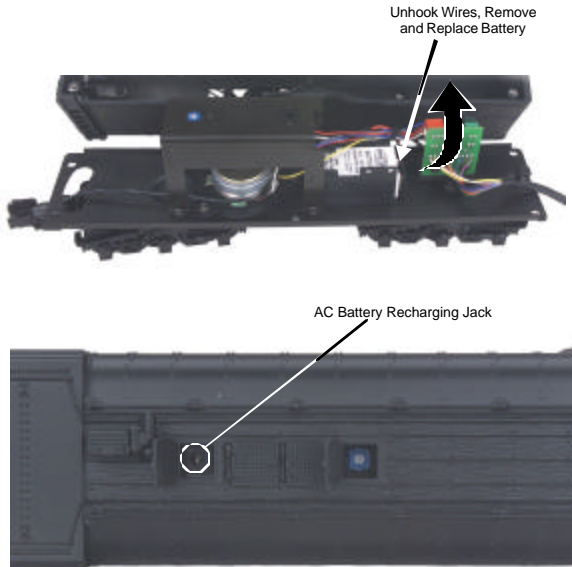
Figure 11: Replacing The Battery And Locating The Battery Recharging Jack
