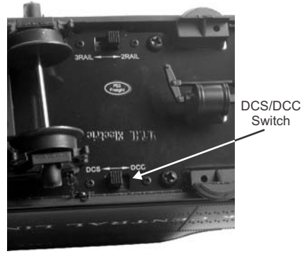
Figure: Changing from DCS to DCC Mode
