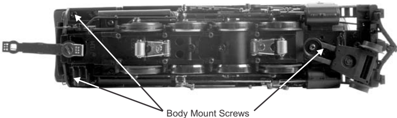
Figure: Removing the Body
