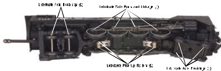
Figure 6. Lubrication Points on the Locomotive
