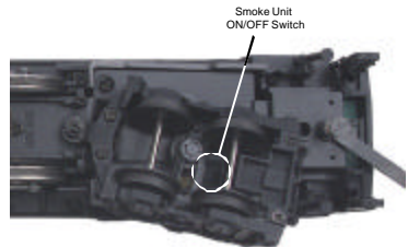
Figure 2: Smoke Unit Switch Location
