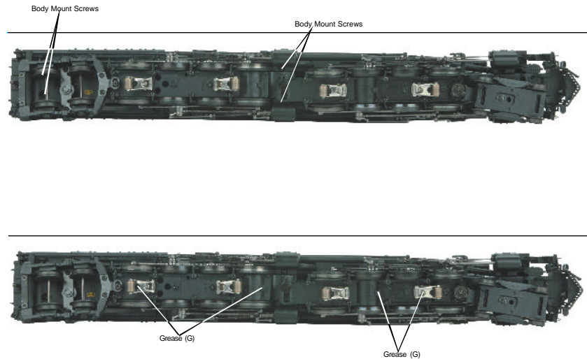
Figure 6: Removing The Body And Lubricating The Grease Points
