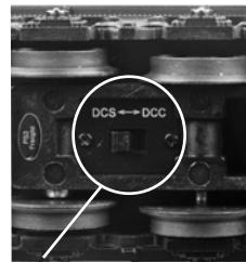
Figure 7: Changing from DCS to DCC Mode
