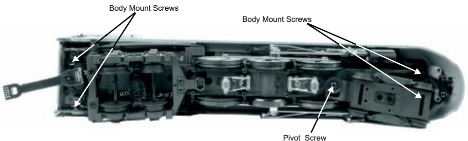
Figure 8: Removing the Body
