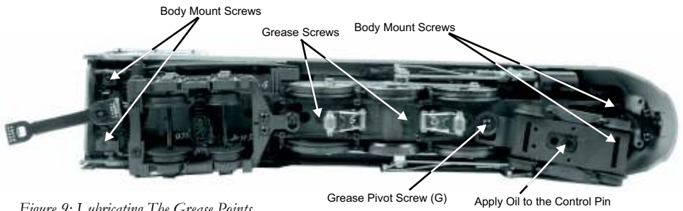
Figure 9: Lubricating The Grease Points
