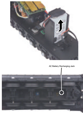
Figure 9: Replacing The Battery And Locating The Battery Recharging Jack
