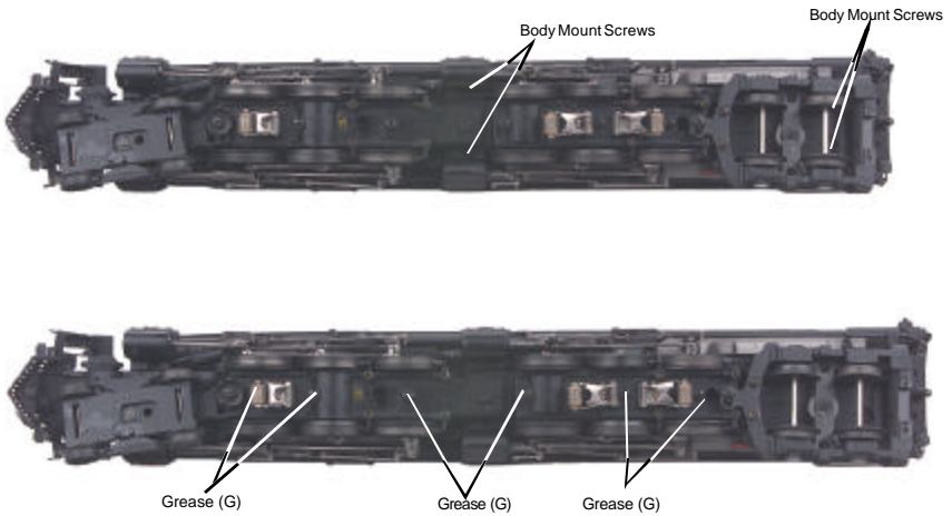
Figure 6: Removing The Body
