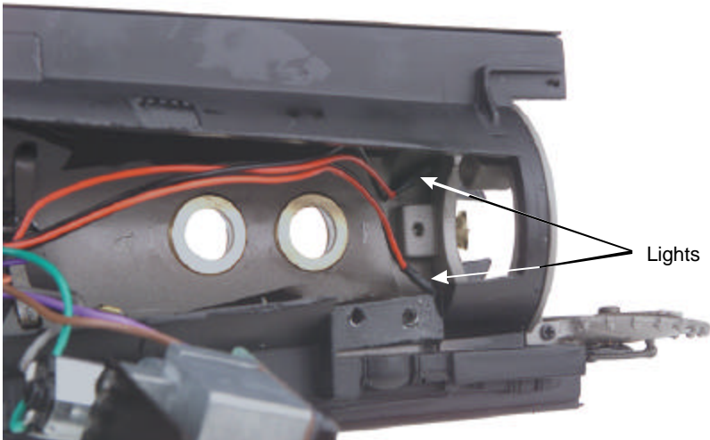
Figure 7: Headlight Wire Harness
