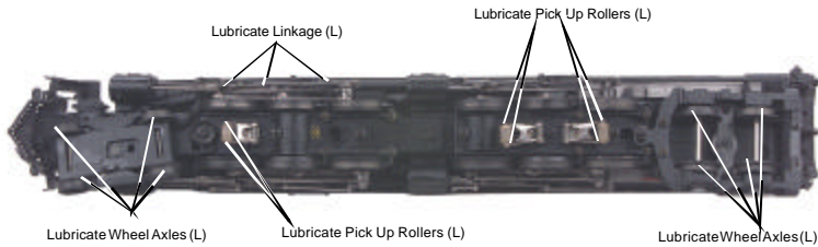
Figure 1. Lubrication Points on the Locomotive
