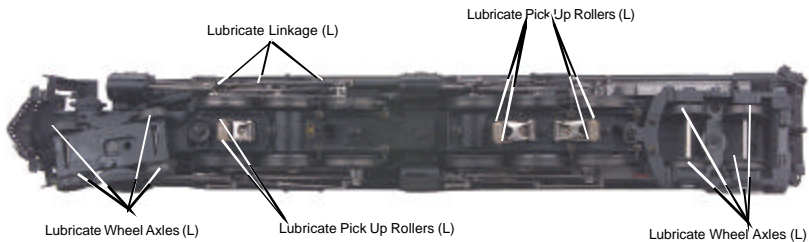
Figure 5: Lubricating The Chassis
