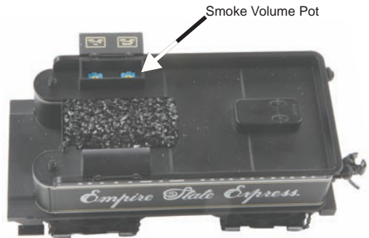
Fig.2: Smoke Unit Switch Location (Inside Tender Hatches)
