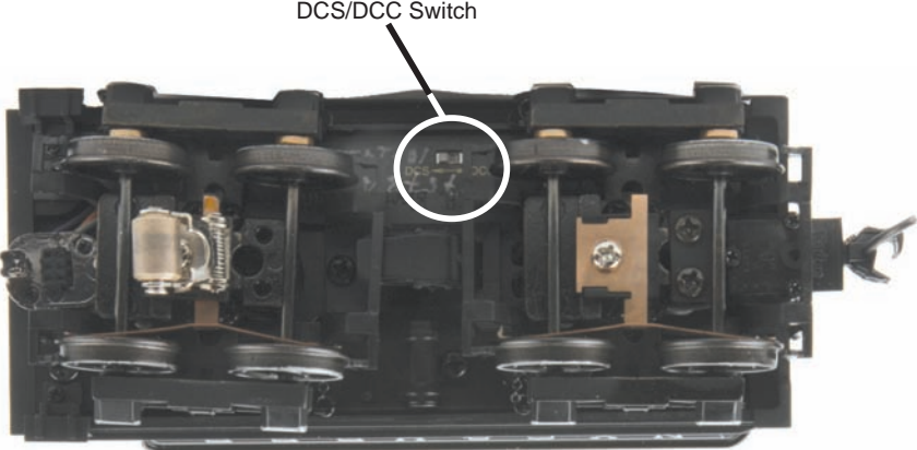
Figure 8: DCS/DCC Switch
