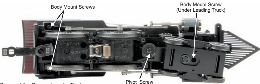
Figure 13: Removing the Body
