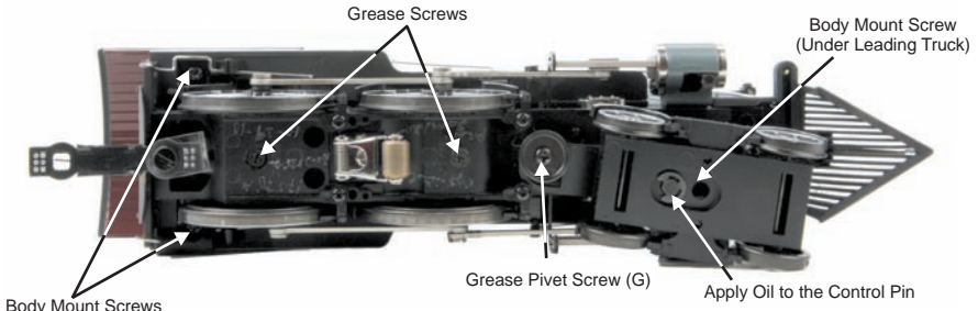
Figure 14: Lubricating The Grease Points
