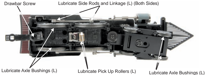
Fig. 12: Lubrication Points on the Locomotive
