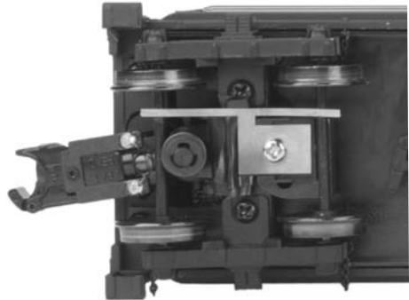
Fig.10: 3-Rail Proto-Coupler
