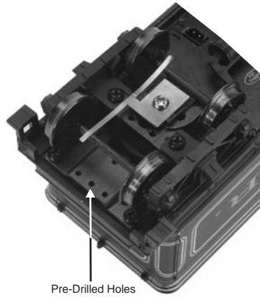
Figure 9: Pre-drilled Kadee® Coupler mounting holes
