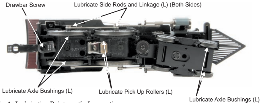
Fig. 1: Lubrication Points on the Locomotive
