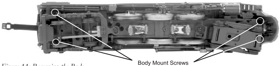
Figure 11: Removing the Body
