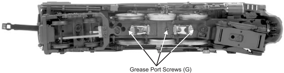
Figure 10: Grease Points
