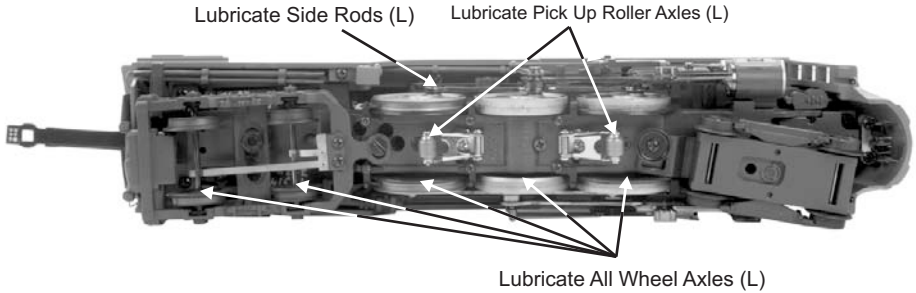
Fig. 9: Lubricating the Locomotive
