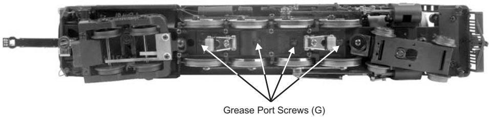
Figure 10: Grease Points
