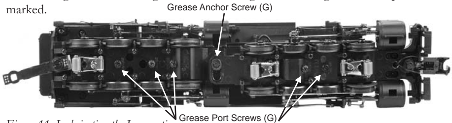
Figure 11: Lubricating the Locomotive Premier 0-8-8-0 Steam Engine
