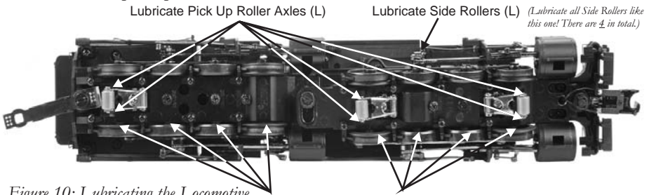
Figure 10: Lubricating the Locomotive
