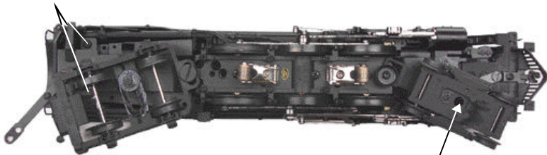
Body Mounting Screw (Through hole in Leading Truck)
