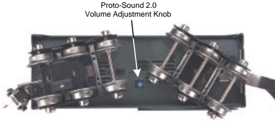
Figure 4: Manually Adjusting The Volume
