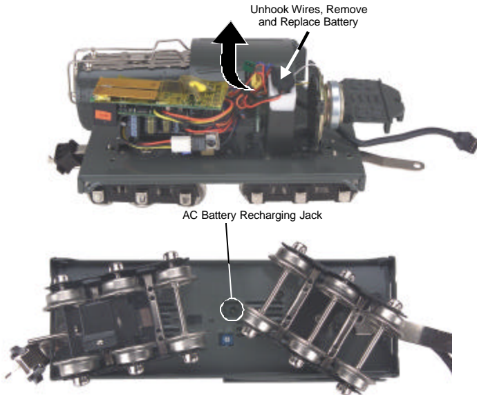
Figure 14: Replacing The Battery And Locating The Battery Recharging Jack
