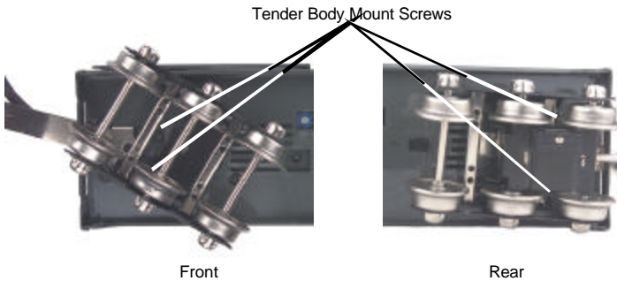
Figure 11: Removing The Tender Body
