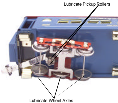
Figure 2: Lubricating The Passenger Car Trucks
