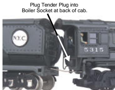
Figure 4: Connecting Tender Harness
