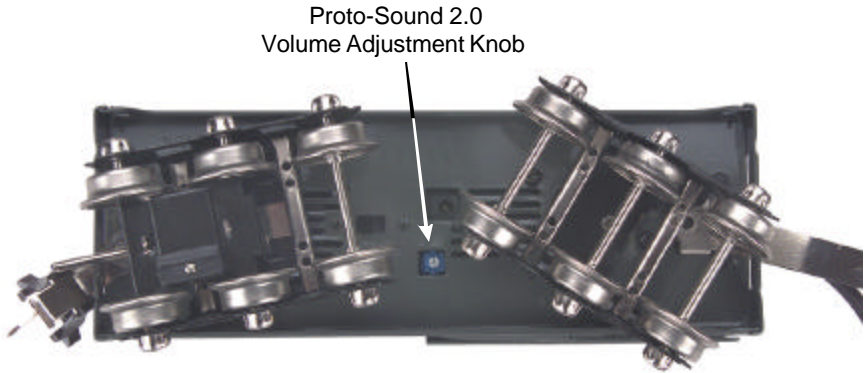
Figure 5: Manual Volume Adjustment
