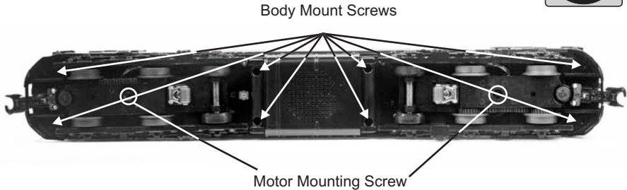
Figure 6: Body Removal Screw Locations and Motor Mounting Screws
