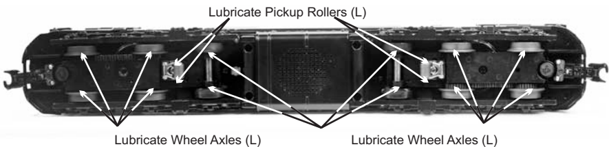
Figure 1. Lubrication Points on the Locomotive
