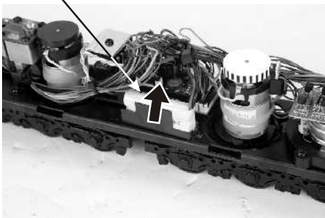
Figure 10. Battery Location.
