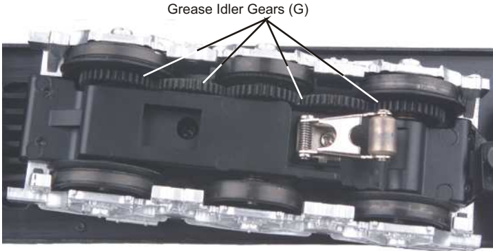
Figure 7. Greasing The Idler Gears
