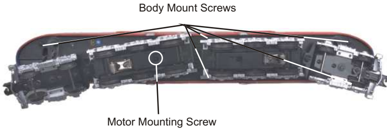
Figure 6. Body Removal Screw Locations
