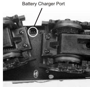
Figure 9. Battery Charger Port location.
