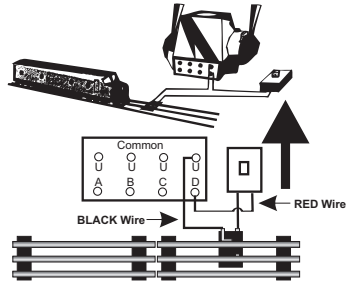
Figure 5: Wiring Up A Bell Button
