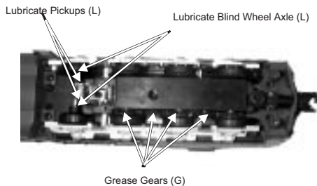
Figure 6: Lubricating The Locomotive Chassis
