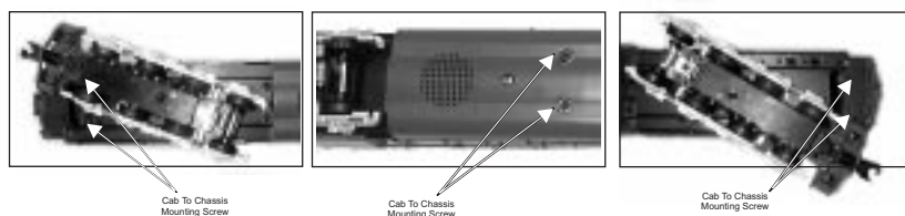
Figure 8: Removing The Body From The Chassis
