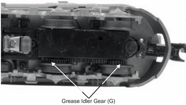
Figure 8: Greasing the Idler Gears
