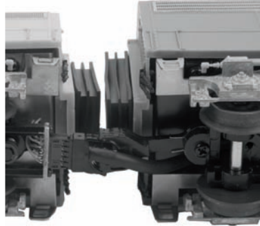
Figure 5: Coupled A and B unit
