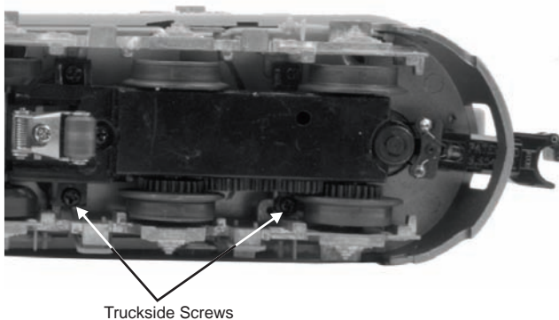
Figure 9: Truckside Screws
