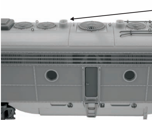
Figure 2: Adding Smoke Fluid
